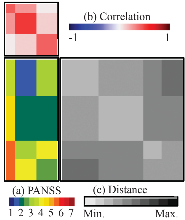
▼圖七 充分統計圖(sufficient statistical graph)
